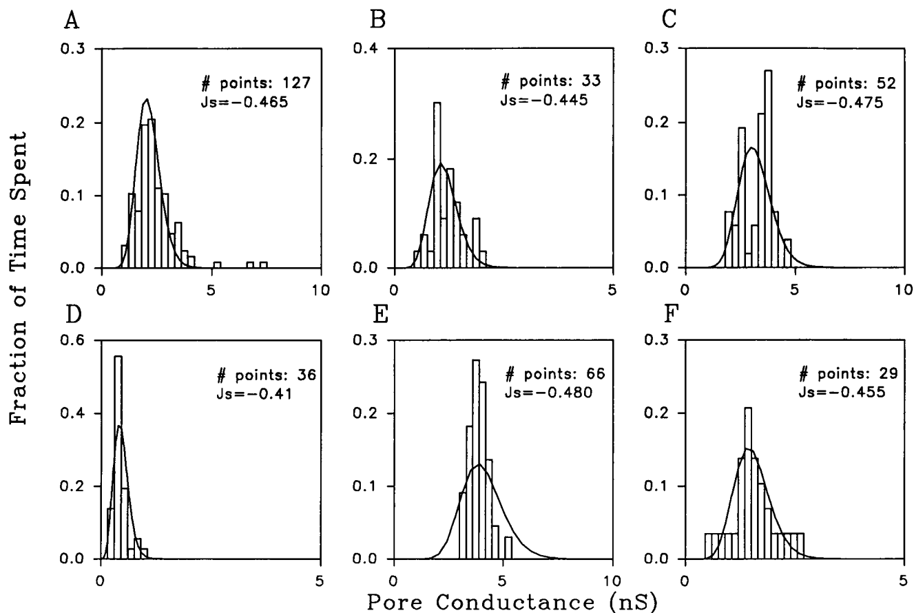
FIGURE 6 Comparison of theoretical predictions with experimental data for irreversible fusion events. Fusion pore conductance histograms (bars) for six irreversible events were fit to theoretically predicted distributions (continuous curves) assuming a pore in a bilayer ( k_c = 1 \times 10^{-12} ergs, h = 2 nm). Tension was 0.1 mN/m and the bin width was 150 pS (A, C, and E) or 300 pS (B, D, and F). The spontaneous curvature for the fits and the number of points in each histograms are specified. The distributions shown in Figs. 6 B and 7 C are from an irreversible and a transient fusion event in the same cell.
