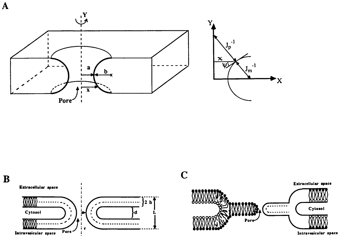
FIGURE 1 (A) Geometry of a pore that is generated by revolving the semicircles (thick curves) about the axis of revolution, Y . a = radius of the narrowest part of the pore; b = radius of the generating semicircles; x = shortest distance between the axis of revolution and a point on the semicircle. Inset shows the same geometry with the angle and radii of curvatures. J_p^{-1} and J_m^{-1} are the parallel and meridional radii of curvature, respectively. \psi(x) is the angle between the tangent to the semicircle at the point (x, y) and the horizontal axis. (B) A pore spanning two bilayers and the space between them. h = monolayer thickness, d = interbilayer distance, L = pore length = 4h + d . (C) A pore spanning the single bilayer formed on hemifusion of the fusing bilayers ( L = 2h ).
